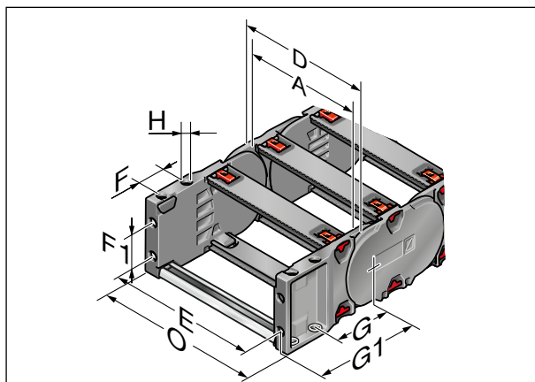
KA 420 Flexible chain bracket
